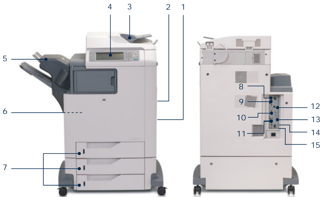
HP Color LaserJet 4730xs mfp front view
